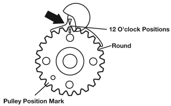
Tool and Crankshaft Pulley with Aligned Timing Mark
